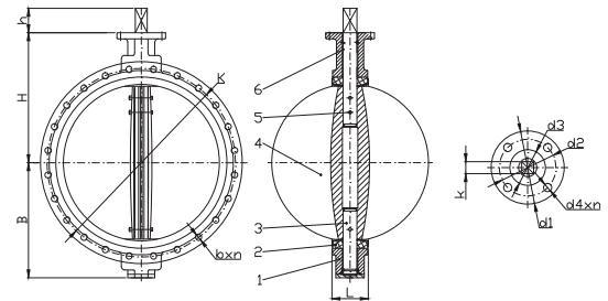
(DN500-DN600)
