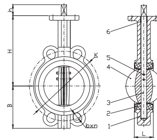
(DN500-DN600)
